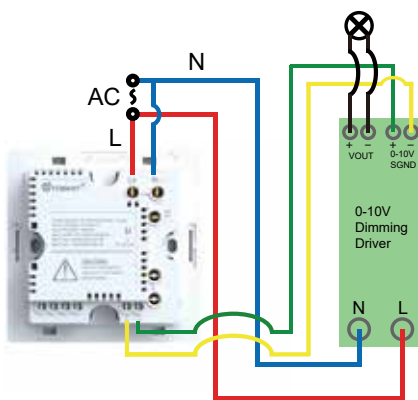
Connection 1: 0-10v Dimming
